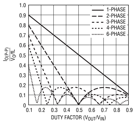
Figure 4. Normalized Peak Output Current vs Duty Factor [ I_{RMS} = 0.3(I_{O(P-P)}) ]
